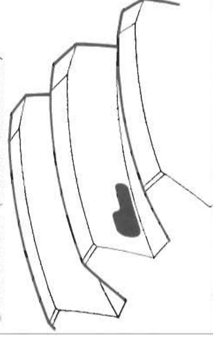
③ INCORRECT (Contact at tooth root)
